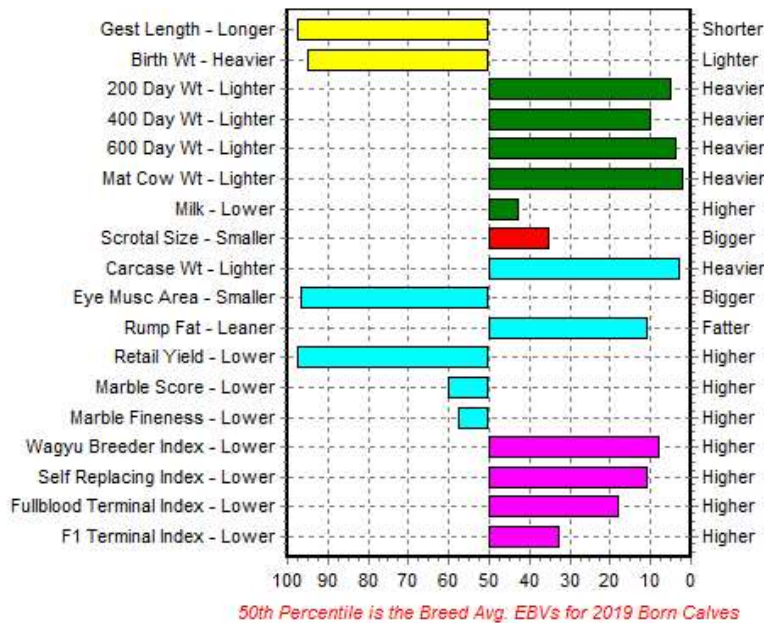
EBV Percentiles for FOCONO K00139
